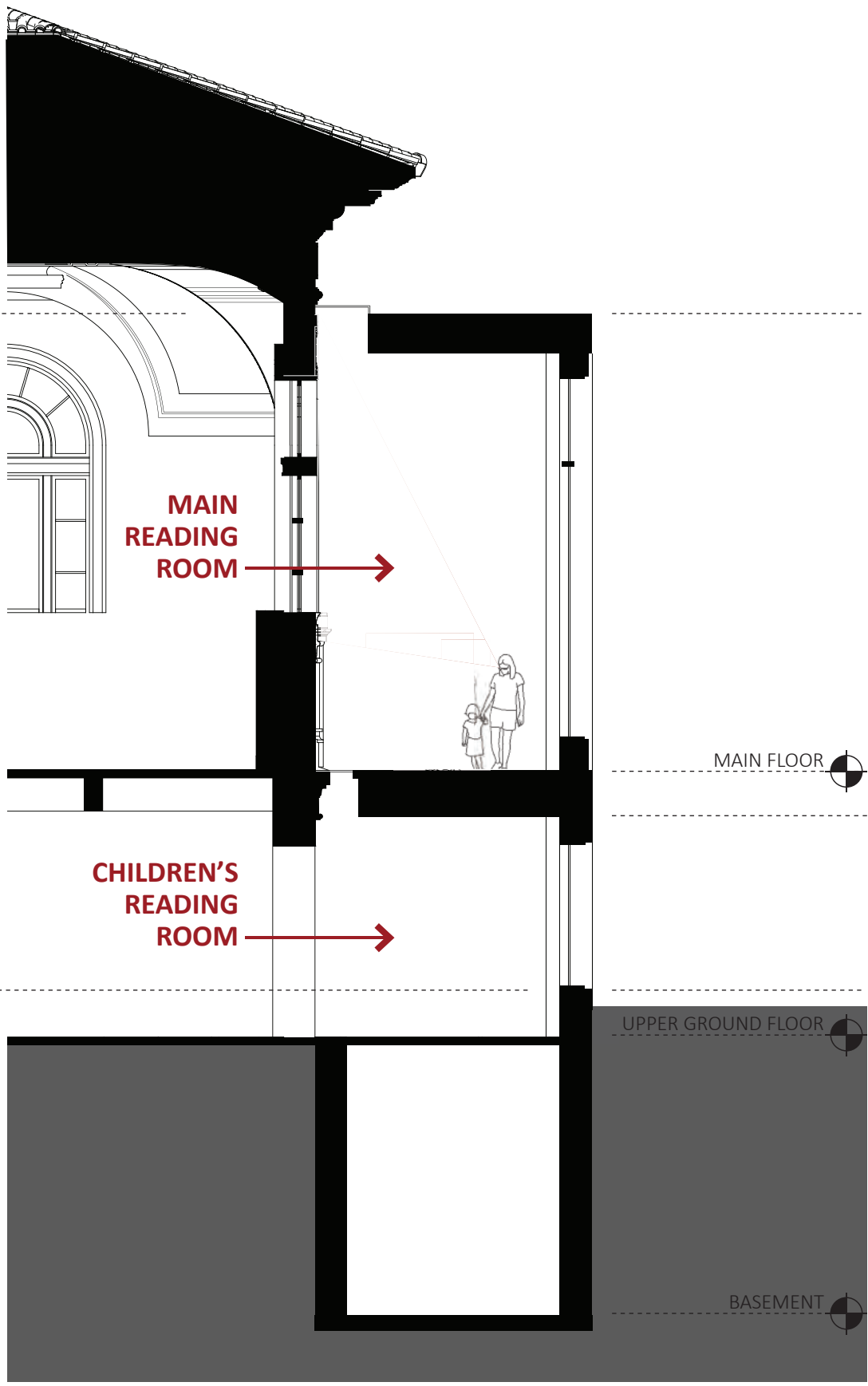
DESIGN STUDIES | CDR - CONCEPTUAL/ PHASE 1 SAN FRANCISCO PUBLIC LIBRARY | MISSION BRANCH LIBRARY | 06.17.19
