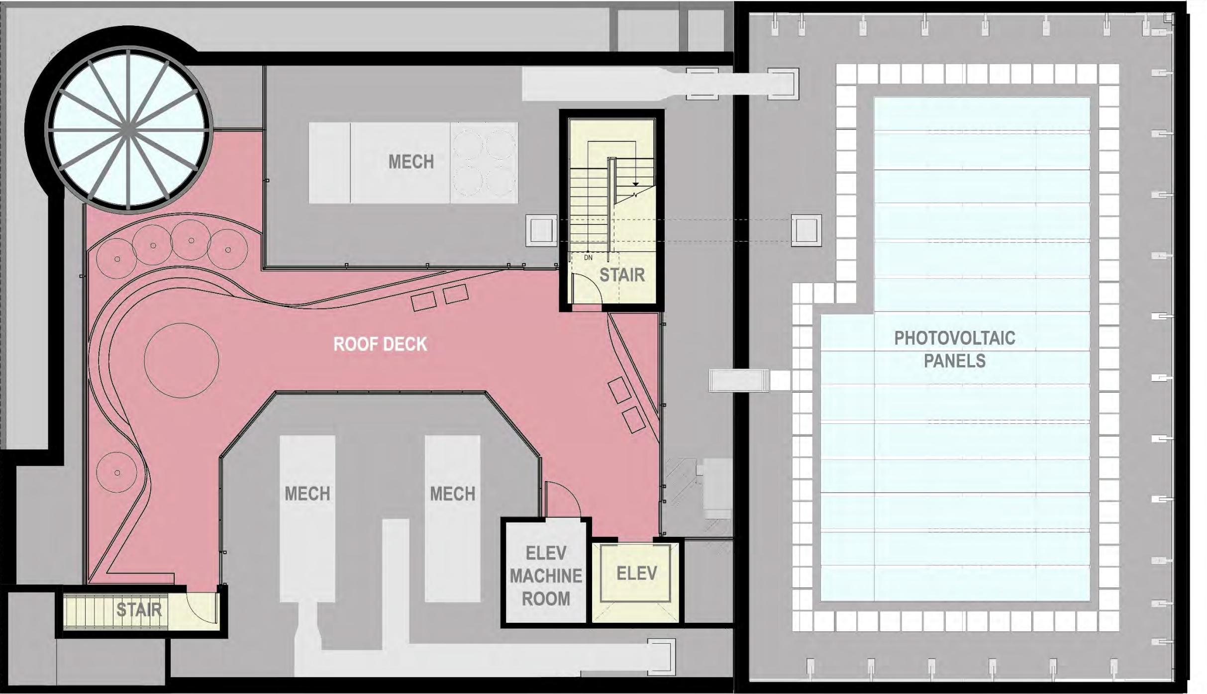
ROOF PLAN
