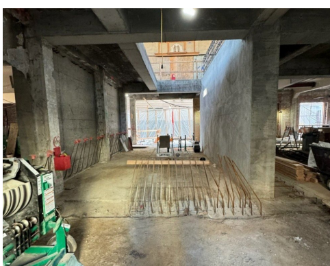
A view of the staircase opening, detailing the reinforcing steel for the stairs.
